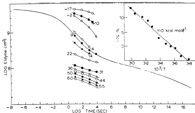
Figure 6. Measured stress relaxation data at the indicated temperatures and the stress relaxation master curve for the Nafion precursor. T_{\text{ref}} = T_g (0.1 Hz) = 10 °C. Many data points have been omitted for clarity. The inset shows a plot of the logarithm of the shift factor against 1/T .
