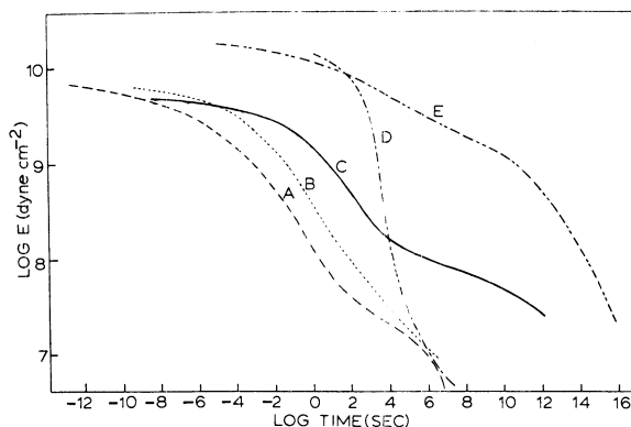
Figure 7. A comparison of the precursor stress relaxation master curve (C) with master curves of other materials: A, Nafion-K ( T_{\text{ref}} = T_g = 213 °C); B, Nafion-H (104 °C); C, Nafion precursor (10 °C); D, polystyrene (102 °C); E, styrene-9.7% sodium methacrylate (130 °C).
